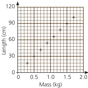
Perfect positive correlation: r_s = +1.0
