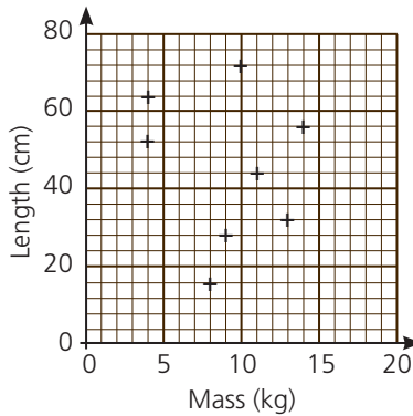
No correlation: r_s = 0
