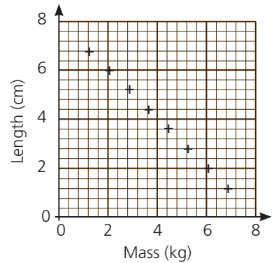
Perfect negative correlation: r_s = -1.0
